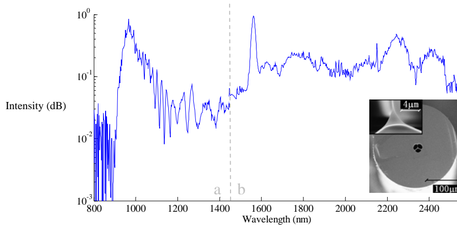
Figure 1: Output Spectra, a) is taken using a fiber coupled Anritsu spectrum analyser, and b) using a Jarrel-Ash monochromator (sensitive to above 2.6 \mu\text{m} ), inset is an SEM of the fiber end-face, figure takes into account spectral response of detection equipment, no continuum signal detected above 2.5 \mu\text{m}
